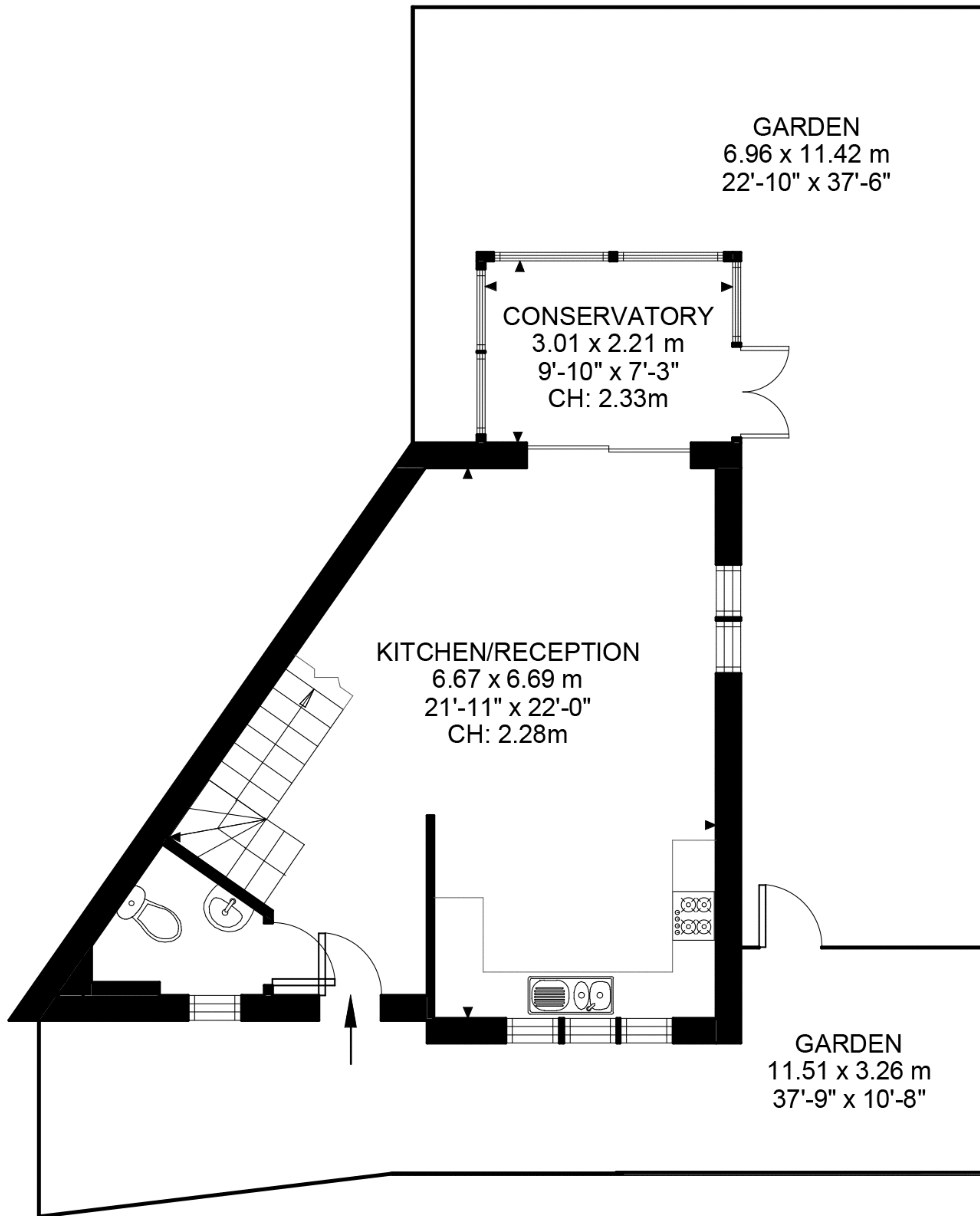
Ground Floor 503 ft 2
